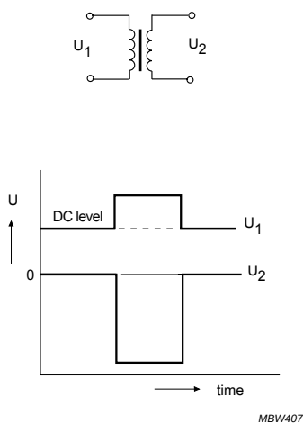
Fig.5 Pulse and general purpose transformer.
