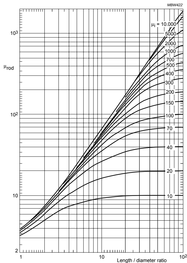
Fig.64 Rod permeability ( \mu_{\text{rod}} ) as a function of length to diameter ratio with material permeability as a parameter.
