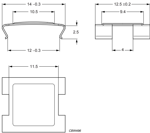
Fig.3 EFD12/6/3.5 mounting clamp.
