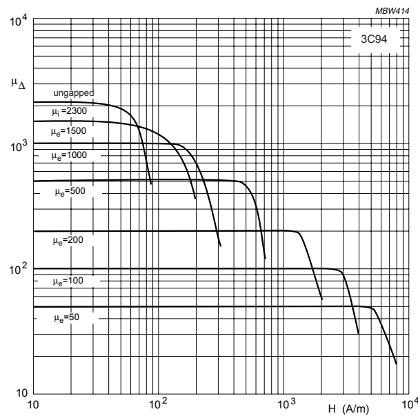
Fig.20 Effect of increased gap length.
