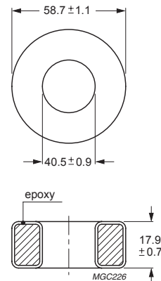
Fig.1 TX58/41/18 ring core.
