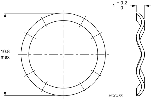
Fig.7 Spring: SPR-P11/7.
