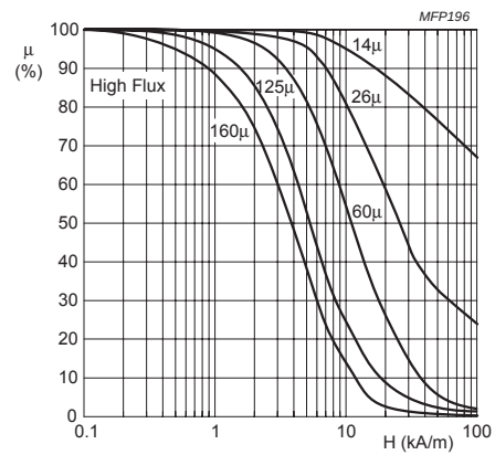
Fig.5 Reversible permeability as a function of magnetic field strength.
