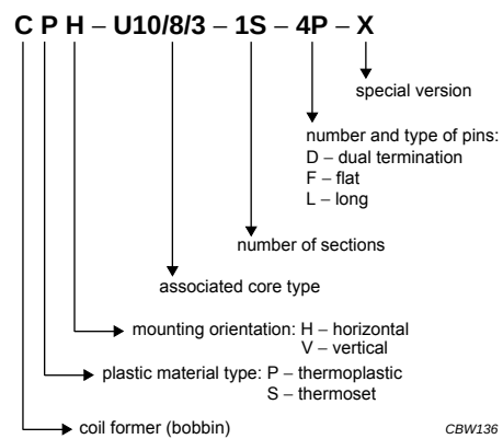
Fig.3 Type number structure for coil formers.
