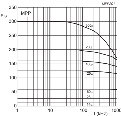
Fig.1 Initial permeability as a function of frequency.
