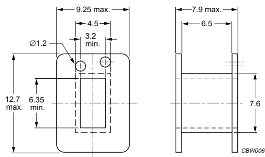
Fig.3 E13/6/6 coil former.
