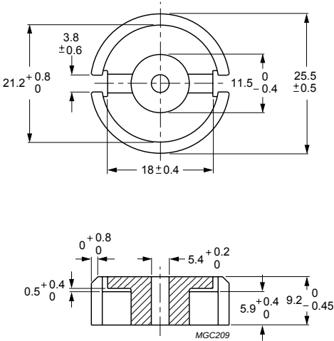
Fig.1 PH26/9.2 core half.
