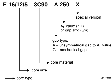
Fig.1 Type number structure for E cores.
