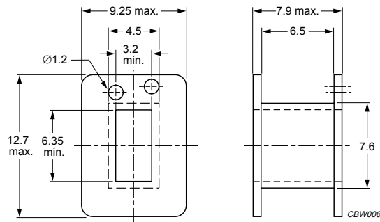
Fig.2 E13/6/6 coil former.
