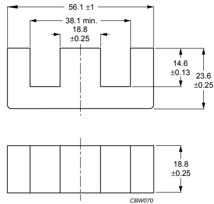
Fig.1 E56/24/19 core half.
