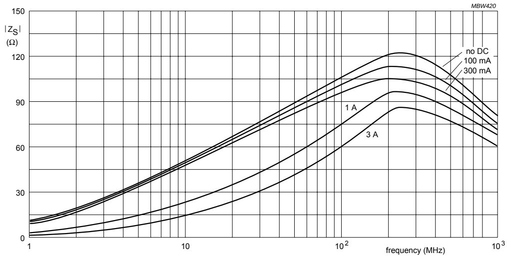
Fig.48 Impedance as a function of frequency at different DC levels for material grade 4S2; bead size 5 \times 2 \times 10 mm.
