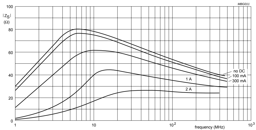
Fig.49 Impedance as a function of frequency at different DC levels for material grade 3S1; bead size 5 \times 2 \times 10 mm.
