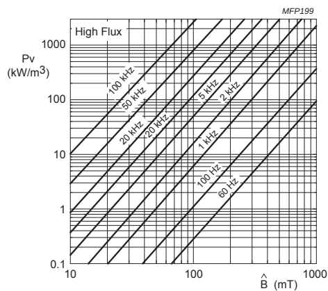
Fig.6 Specific power loss as a function of peak flux density with frequency as a parameter for material 14μ.
