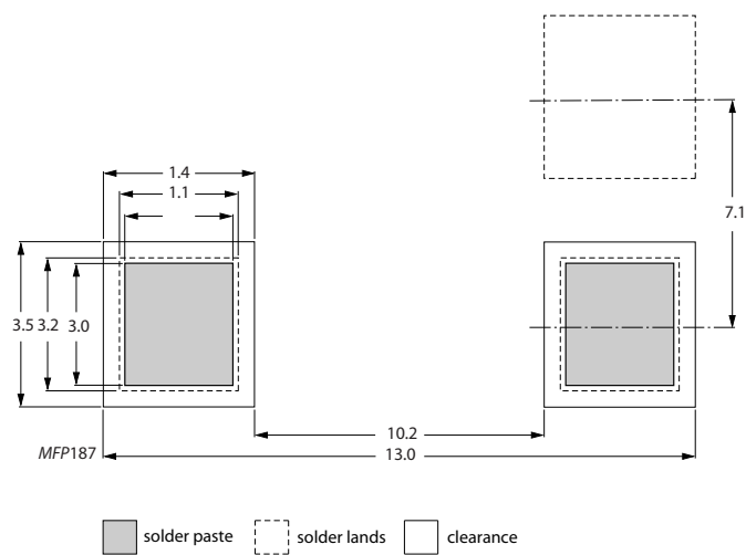
Fig.3 Recommended solder lands
