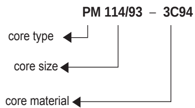
Fig.1 Type number structure for PM cores.
