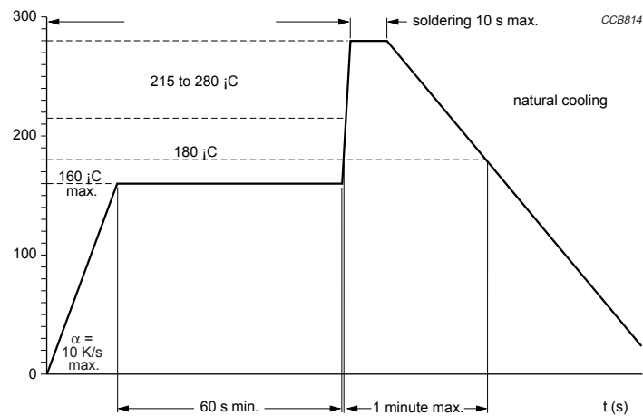
Fig.2 Recommended temperature profile for reflow soldering.
