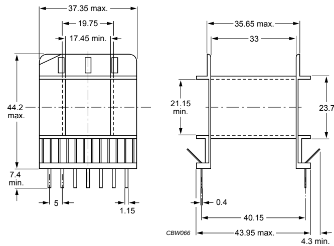
Fig.4 E55/28/21 coil former; 14-pins.
