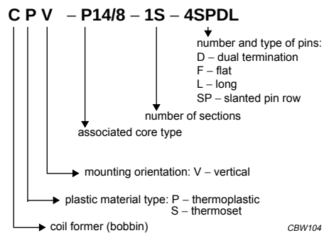
Fig.2 Type number structure for coil formers.
