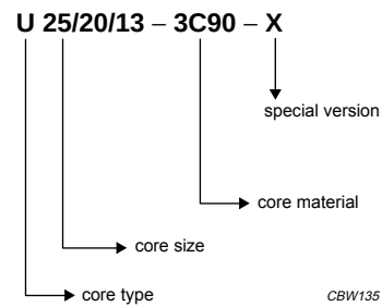
Fig.1 Type number structure for U cores.
