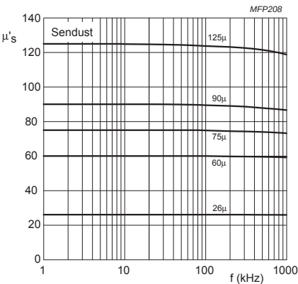
Fig.1 Initial permeability as a function of frequency.
