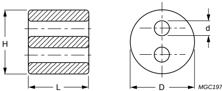
Fig.1 Multihole core circular (MHC2).
