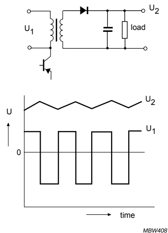
Fig.6 Power transformer application.
