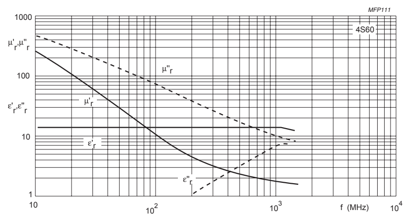
Fig.4 Complex permeability and permittivity as a function of frequency (high end).
