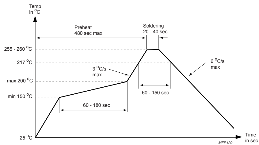
Fig.5 Reflow soldering.
