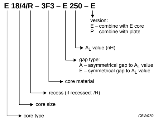
Fig.1 Type number structure for E cores.
