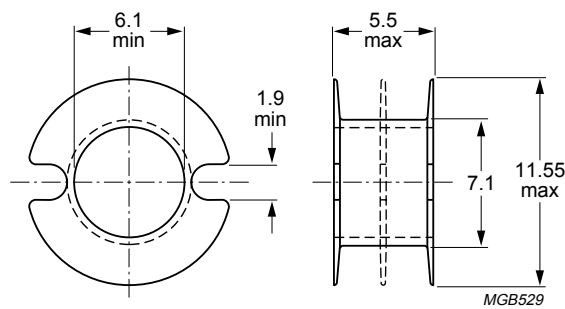
Fig.4 Coil former CP-P14/8-A.
