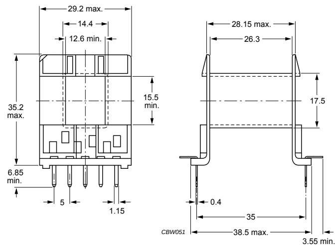
Fig.4 E42/21/15 coil former; 10-pins (A).
