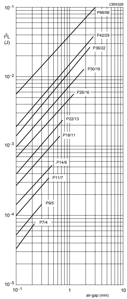
Fig.28 I^2L graph for P cores.
