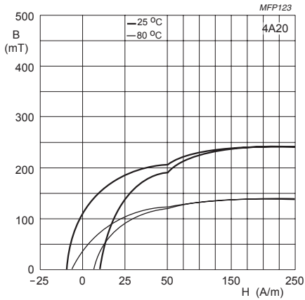
Fig.3 Typical B-H loops.
