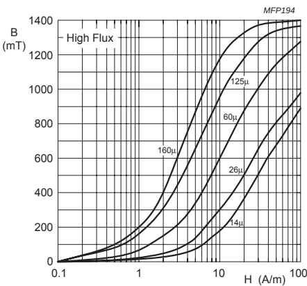
Fig.3 Typical B-H curves.
