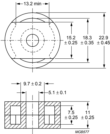
Fig.1 PT23/11 core set.
