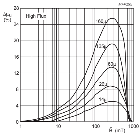
Fig.4 Amplitude permeability as a function of peak flux density.
