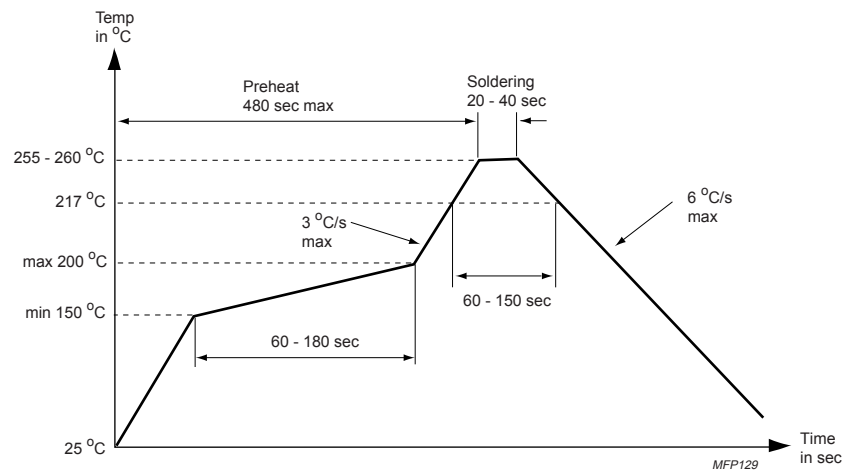
Fig.3 Reflow soldering.
