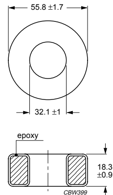
Fig.1 TX55/32/18 ring core.
