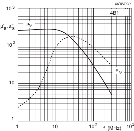
Fig.1 Complex permeability as a function of frequency.
