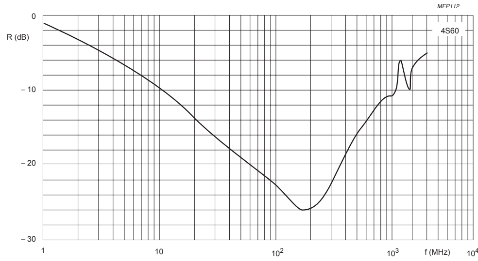
Fig.5 Reflectivity at normal incidence as a function of frequency.
