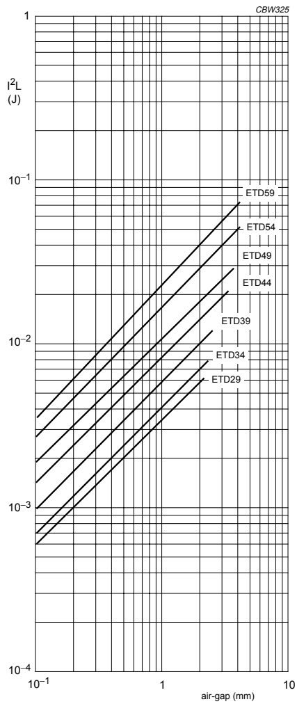
Fig.27 I^2L graph for ETD cores.
