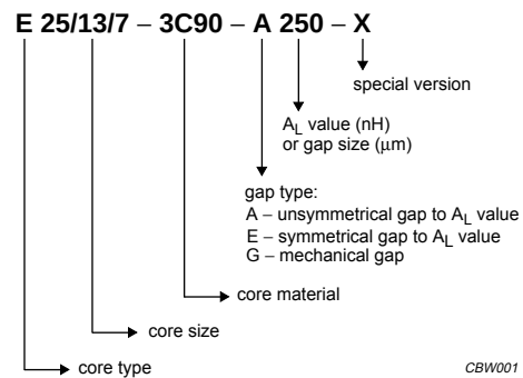
Fig.1 Type number structure for cores.
