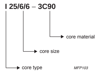
Fig.2 Type number structure for I cores.
