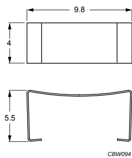
Fig.3 ER9.5/2.5/5 clamp.
